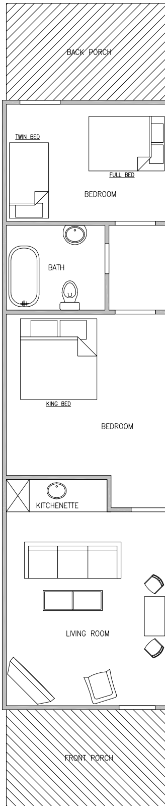
FLOOR PLAN SERENITY COTTAGE
